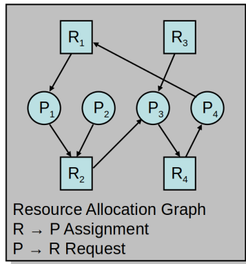
Figure 2: Resource Allocation Graph
