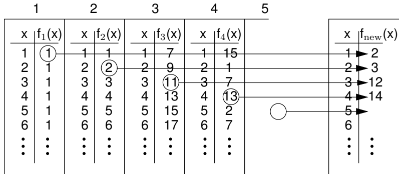
Figure 17.6 Illustration for the argument that the number of integer functions is uncountable.
