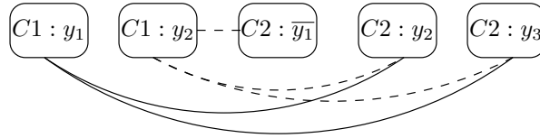
Figure 17.4 The graph that results from converting the boolean expression B = (y_1 + y_2) \cdot (\bar{y}_1 + y_2 + y_3) . Literals from the first clause are labeled C1, and literals from the second clause are labeled C2. There is an edge between every two pairs of vertices except when both vertices represent instances of literals from the same clause, or a negation of the same variable. Thus, the vertex labeled C1 : y_1 does not connect to the vertex labeled C1 : y_2 (because they are literals in the same clause) or the vertex labeled C2 : \bar{y}_1 (because they are opposite values for the same variable).
