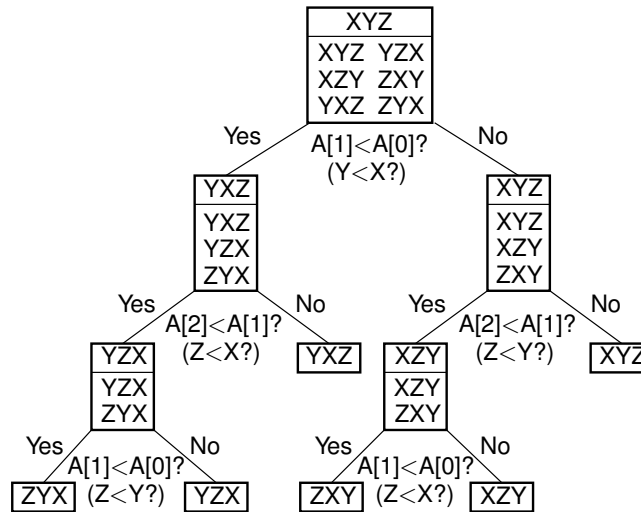
Figure 7.14 Decision tree for Insertion Sort when processing three values labeled X, Y, and Z, initially stored at positions 0, 1, and 2, respectively, in input array A.
