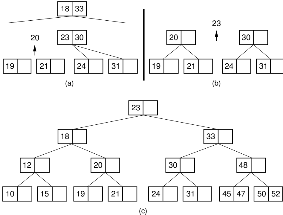
Figure 10.13 Example of inserting a record that causes the 2-3 tree root to split. (a) The value 19 is added to the 2-3 tree of Figure 10.9. This causes the node containing 20 and 21 to split, promoting 20. (b) This in turn causes the internal node containing 23 and 30 to split, promoting 23. (c) Finally, the root node splits, promoting 23 to become the left record in the new root. The result is that the tree becomes one level higher.
