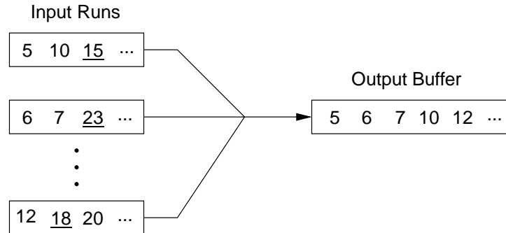
Figure 8.11 Illustration of multiway merge. The first value in each input run is examined and the smallest sent to the output. This value is removed from the input and the process repeated. In this example, values 5, 6, and 12 are compared first. Value 5 is removed from the first run and sent to the output. Values 10, 6, and 12 will be compared next. After the first five values have been output, the “current” value of each block is the one underlined.
